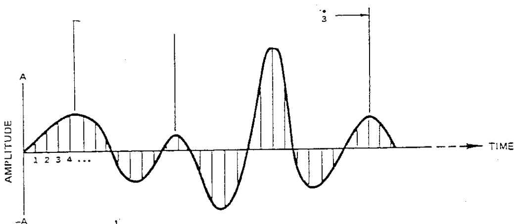
FIGURE 72 Deep-water wave-record sample, showing construction for statistical analysis.
