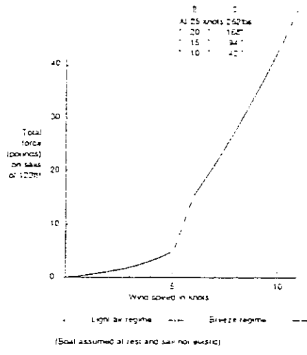
Fig 5.2 Change of sail force with wind speed
