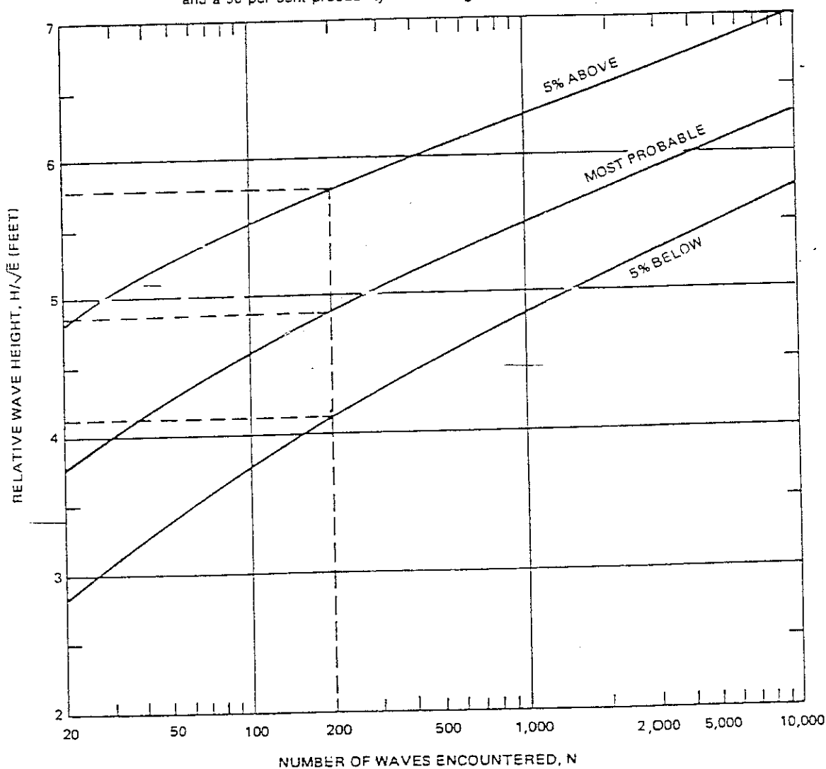
FIGURE 74 Extreme wave probability increases with the number N of waves encountered. Example shows that there is a 5 per cent chance that the highest of 200 successive waves, will exceed H = 5.8\sqrt{E} , the same chance that it will be lower than H = 4.1\sqrt{E} , and a 90 per cent probability of its being in between.
